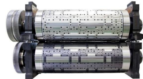
Cutting - Cylinders
